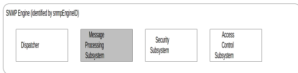
Figur: SNMP MPS [3]
