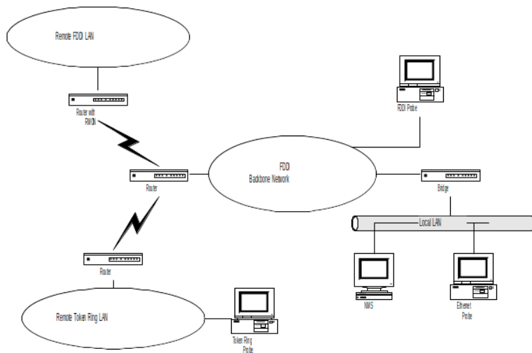
Figure 8.1 Network Configuration with RMONs
