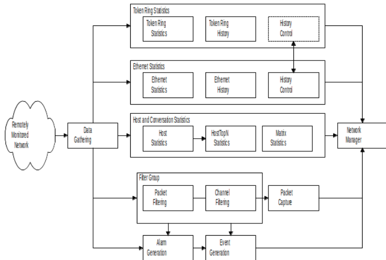
Figure 8.3 RMON Groups and Functions
