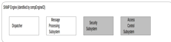
Figur: SNMP SM [3]
