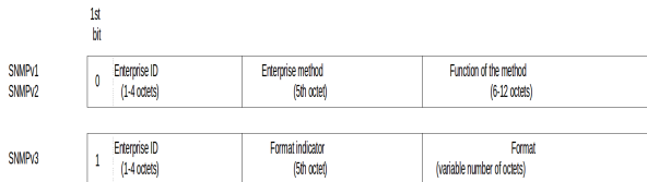
Figur: Engine ID [3]
